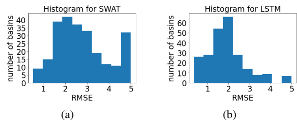
Figure 1: RMSE distribution by (a) the process-based SWAT model and (b) the global LSTM over all the basins. The rightmost bin in each figure represents the basins with \text{RMSE} \geq 5 .
