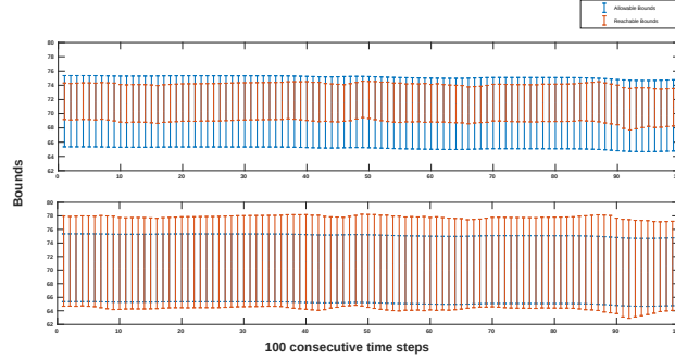
Fig. 2: Allowable (blue) and reachable (red) bounds for battery SOC dataset for 100 consecutive time steps and 2 different SFAI noise values 1% (upper), and 2.5% (lower) respectively
