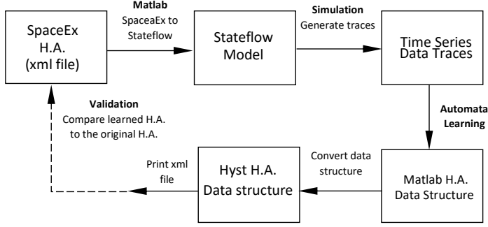
Fig. 2. Overview of the validation of the proposed framework for the method described in this paper. A given hybrid automaton is specified in the SpaceX/HyST [7, 21] format, automatically translated to a Simulink/Stateflow model using HyST [6, 7], simulated to generate time series data (traces). The hybrid automata learning framework is then applied to these traces, and a learned hybrid automaton is generated in the SpaceX/HyST format, and simulated again to generate traces to validate the learned model's behaviors against the original model's behaviors.
